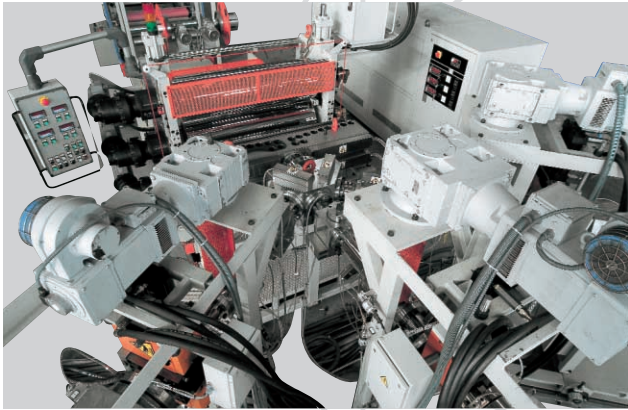
PET-foil extrusion line with vertical calender. Throughput over 600 Kg/h. Detail of the 5-layer co-extrusion unit.
