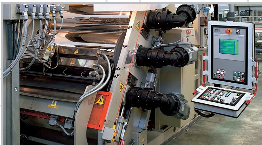
PET-foil extrusion line with throughput over 900 Kg/h. Detail of the new computerized control panel assembled directly on the sloping calender unit.
